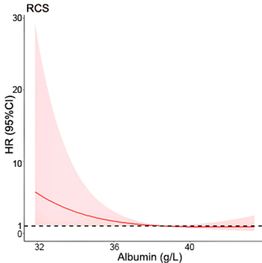
Figure 2 Hazard ratio function for albumin to negative conversion rate. Abbreviations: RCS, restricted cubic splines; HR, hazard ratio; CI, confidence interval.
