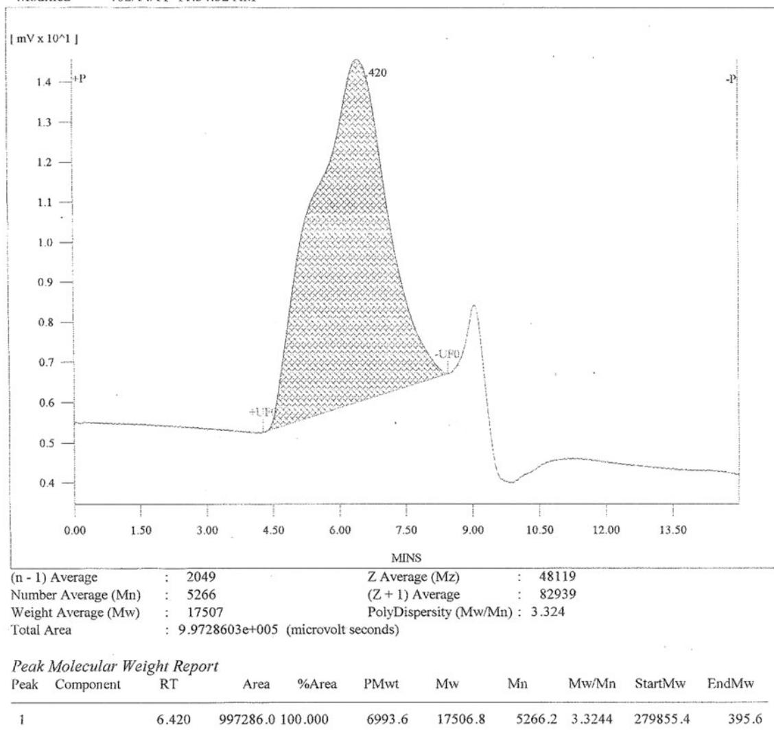
Fig. 2 Gel permeation chromatogram of cPCL showing molecular weight of synthesized polymer as 17,507 Da
