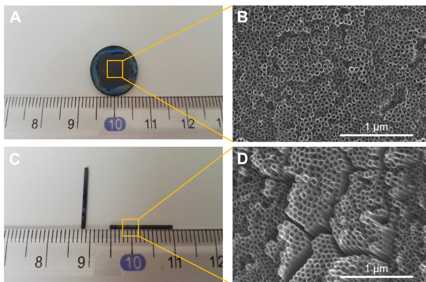
Figure 2 (A and C) Macroscopic images of Ti 2 %Ag-NT used in vitro and in vivo . (B and D) SEM images of nanotubes formed on the surface of Ti 2 %Ag-NT. Abbreviations: NT, nanotubes; SEM, scanning electron microscope.
