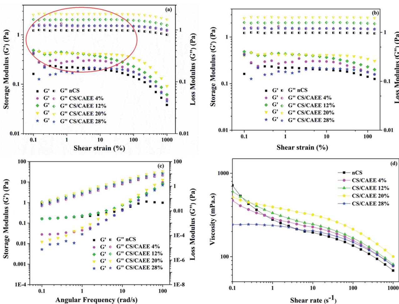
Fig. 8 (a) Strain sweep parameters of the G' and G'' moduli at f = 1 Hz, (b) emphasizing the LVR, (c) frequency sweep parameters of the G' and G'' moduli, and (d) flow curves of the developed biocomposite films together with the control.
