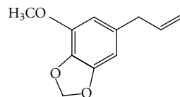
Myristicin
