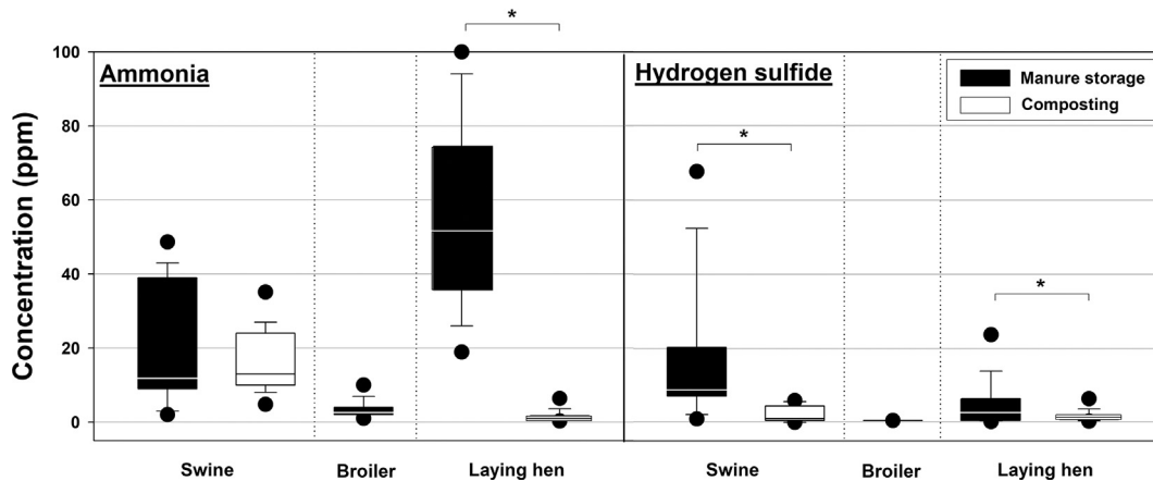
Fig. 2. Concentration of ammonia and hydrogen sulfide at manure storage facilities and composting facilities; the line values of each boxplot indicate mean (line within the box), 25th and 75th percentiles (bottom and top of the box, respectively), 10th and 90th percentiles (lower and upper bars on the whisker, respectively), and outliers (black circles). *, p < 0.0001 .
