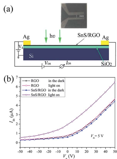
Fig. 4 (a) The optical image and schematic of a representative device. (b) The transfer characteristics ( I_{ds}-V_g ) of the photodetectors based on RGO and SnS/RGO in the dark and under visible-light illumination, P = 10 \text{ mW cm}^{-2} .
