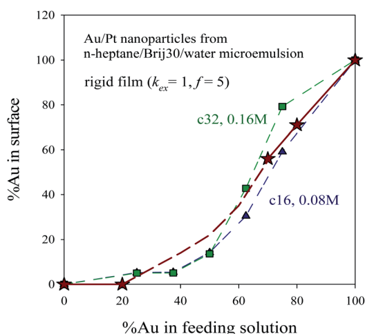
Fig. 8 %Au at the surface versus %Au in feeding solution. Synthesis conditions: rigid film ( k_{ex} = 1 , f = 5 ), \langle c \rangle = 32 reactants/micelle \sim 0.16 M (green squares) and \langle c \rangle = 16 reactants/micelle \sim 0.08 M (blue triangles). Stars represent experimental data of Au/Pt nanocatalysts synthesized in a n -heptane/Brij30/water microemulsion, taken from ref. 12. Lines are only guides to the eye.
