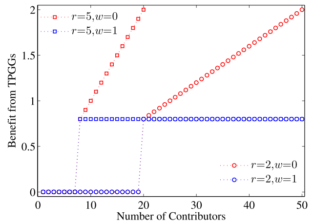
Figure 1 | Diagrams illustrating four examples of TPGG, whose dynamics outcomes are closely related to the model parameter involved. Parameters here: N = 50 , T^* = 40 . The x-axis is indexed by the number of contributors (including cooperators and insured cooperators), and the y-axis represents the individual benefits from TPGG. Results show that, when r = 5 , individuals can gain positive benefits from TPGG if there are at least 8 contributors. When r = 2 , at least 20 contributors in one TPGG are needed to bring each participant with positive benefits. As mentioned, varying the parameter \omega can transverse the model smoothly from scenario I (i.e. \omega = 1 ) to scenario II (i.e. \omega = 0 ) about the payoff functions in the TPGG after the threshold point has already been reached. In between the two extremes, we obtain a mixed situation of the payoff distribution rules in the threshold public goods system.
