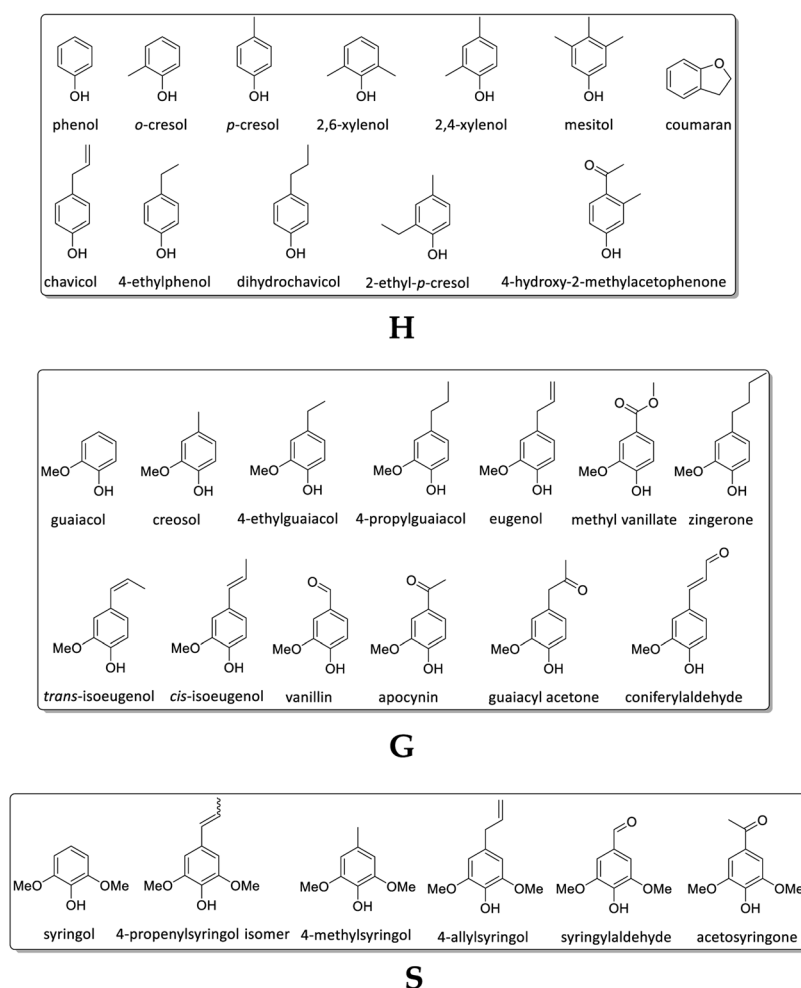
Fig. 8 Detected Py-GC/MS fragments attributed to the three subunits (G, H and S).
