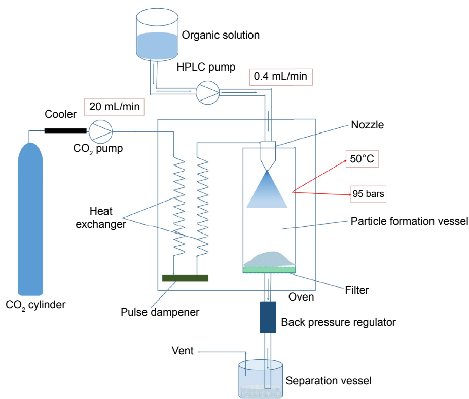
Figure 2 The schematic diagram of the supercritical fluid process. Abbreviation: HPLC, High-performance liquid chromatograph.
