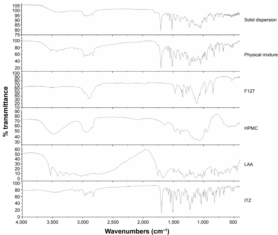
Figure 5 The FT-IR spectra of LAA, ITZ, F127, HPMC, and SD particles.
