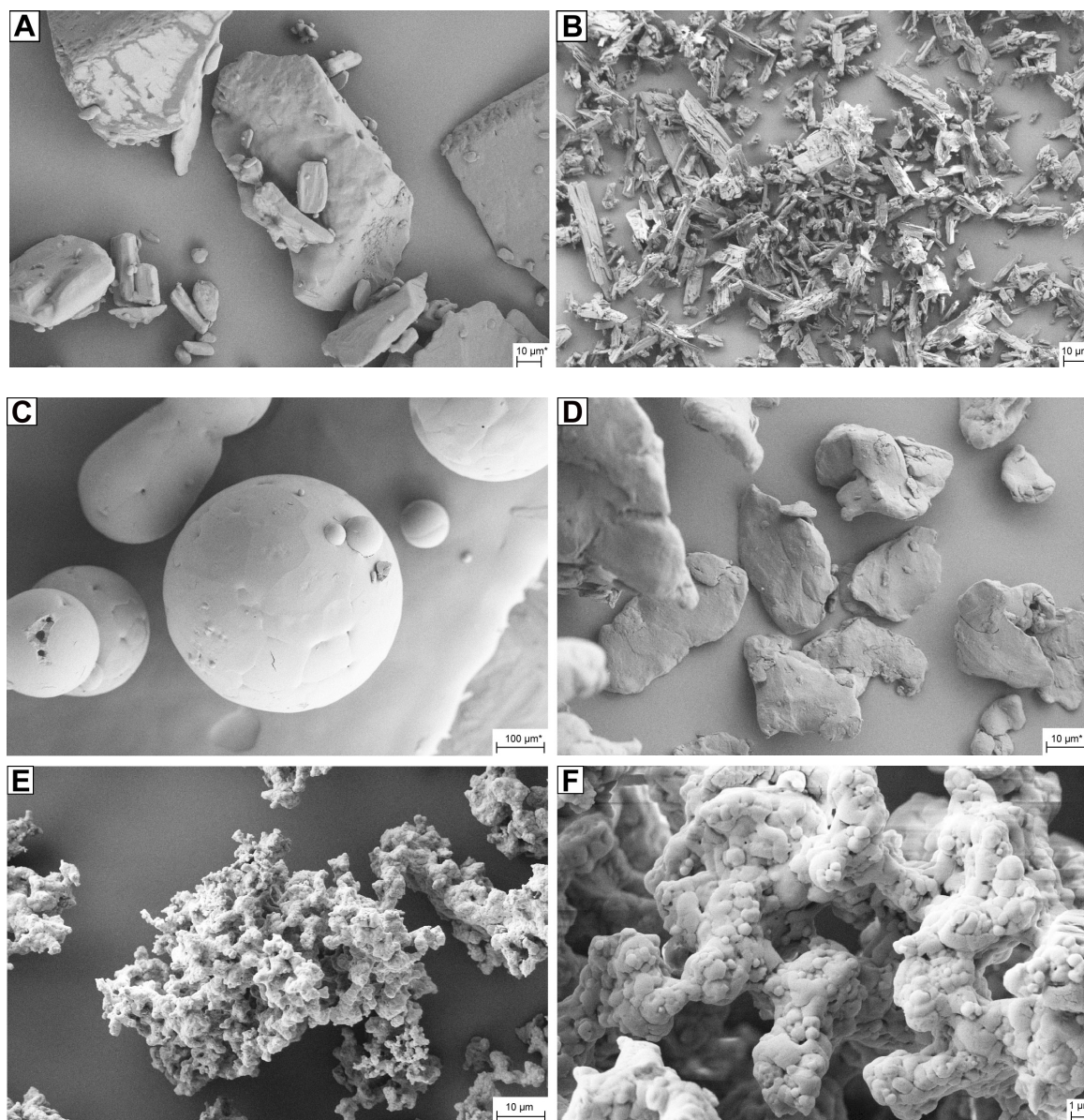
Figure 3 The surface morphology of LAA (A), ITZ (B), FI27 (C), HPMC (D), SD particles (E and F) observed by SEM.
