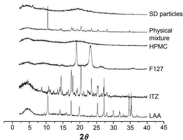
Figure 4 The powder X-ray diffractograms of LAA, ITZ, F127, HPMC, and SD particles.
