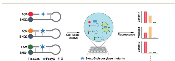
Fig. 2 Illustration of the 8-oxoG glycosylase-screening platform.
