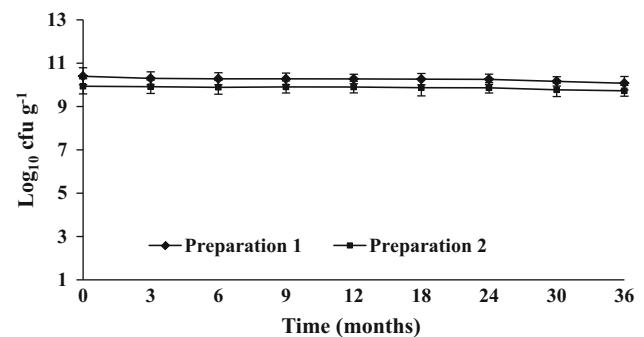
Fig. 7 Viability of B. coagulans MTCC 5856 during the storage at room temperature ( 25 \pm 2 \text{ }^\circ\text{C} with RH 60 \% \pm 5 \% ). Two standardized commercial preparations equivalent to 15 \times 10^9 (preparation 1) and 6 \times 10^9 \text{cfu g}^{-1} (preparation 2) were studied. Average means of spore viable counts are expressed in \log_{10} \text{cfu g}^{-1} . Each time point represents the mean \log_{10} standard deviations ( \pm\text{SD} ) of three different experiments performed in duplicate
