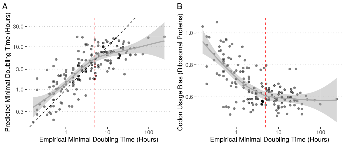
Fig. 1. Predictions from gRodon accurately reflect prokaryotic growth rates, with the caveat that (A) gRodon underestimates doubling times when growth is very slow due to (B) a floor on CUB reached in slow-growth regimes. Vertical dashed red lines at 5 h indicate where the CUB vs. doubling-time relationship appears to flatten. The black dashed line in A is the x = y reference line.
