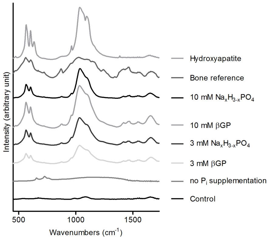
Figure 4. FT-IR spectra. FT-IR spectra ( 450\text{--}1750\text{ cm}^{-1} ) of samples cultured in different osteogenic induction or control media ( n = 1 ) show the characteristic hydroxyapatite bands and the bands characteristic of the organic matrix of bone. doi:10.1371/journal.pone.0065943.g004
