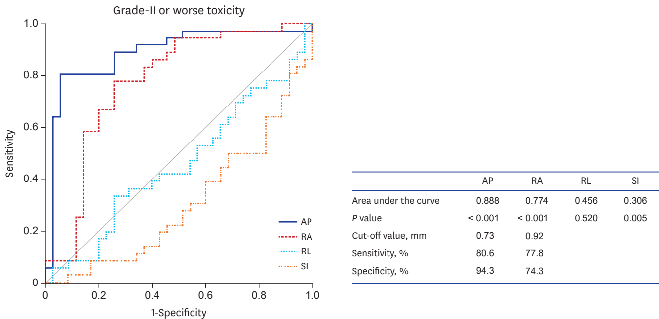
Fig. 3. ROC curves for prostate motion along three translational axes (AP, RL, and SI) and overall radial magnitude to predict grade-II or worse rectal and bladder toxicities. The straight diagonal line on which the sensitivity is equal to 1 in specificity is drawn for reference. Statistical analysis results related to the graph are shown in the inset table.
