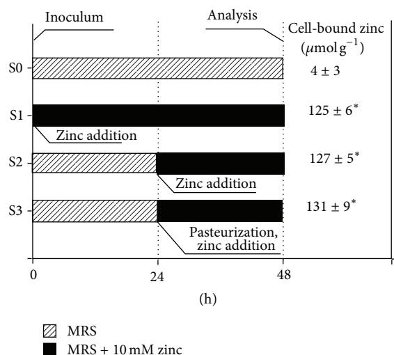
FIGURE 1: Time course of trials S0, S1, S2, and S3 and corresponding cell-bound zinc after 48 h. Dashed bar indicates incubation in MRS broth; black bar indicates incubation in MRS broth + 10 mmol L -1 ZnSO 4 . Values are means from three separate experiments ± SD. Means sharing a common superscript do not differ ( P > 0.05 ).
