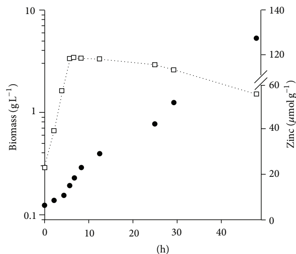
FIGURE 2: Batch culture of Lactobacillus acidophilus WC 0203 in MRS broth containing 10 mmol L -1 . Symbols: □, biomass dry weight; ●, cell-bound zinc.
