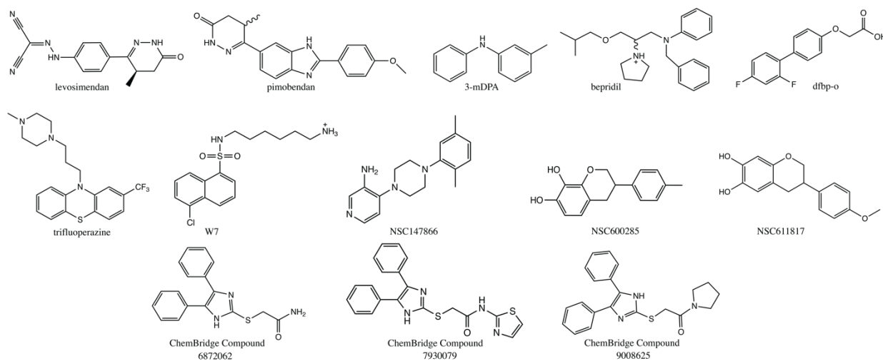
Figure 1. 2D structure of known cNTnC Ca 2+ sensitivity modulators.
