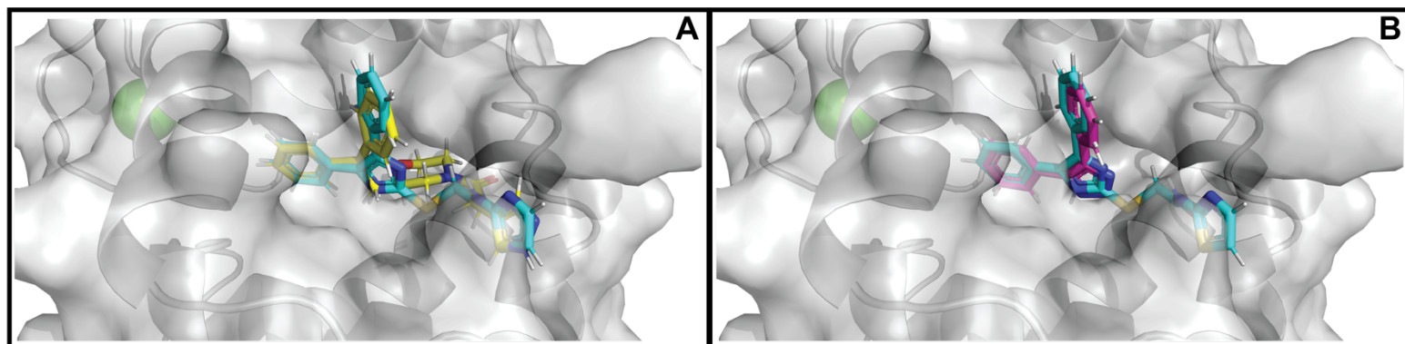
Figure 5. Docked poses of Ca 2+ modulators in cNTnC hydrophobic pocket. PDB 1LXF model 6 is shown in gray surface representation with the protein backbone explicitly shown in cartoon representation, calcium sensitizer 2-[(4,5-diphenyl-1H-imidazol-2-yl)thio]-N-1,3-thiazol-2-ylacetamide shown in cyan overlaid with compound 16 shown in yellow (panel A ) and compound 2 shown in magenta (panel B ).
