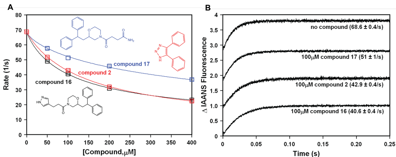
Figure 4. Effect of the hit compounds on the \text{Ca}^{2+} dissociation rate from the chimera. Panel (A) shows the plot of the apparent rates of \text{Ca}^{2+} dissociation from the chimera in the presence of increased concentration of compounds 2, 16 or 17. Each data point represents an average of at least three measurements \pm standard error. Data were fit with an asymmetric sigmoid curve. Panel (B) shows representative stopped-flow traces as \text{Ca}^{2+} is removed from the chimera in the absence or presence of 100 \mu\text{M} of compounds 2, 16 or 17. The traces have been normalized and staggered for clarity.
