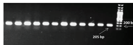
FIGURE 2: Agarose gel electrophoresis of nested PCR products from clinical specimens using species-specific oligonucleotide pairs for P. falciparum .
