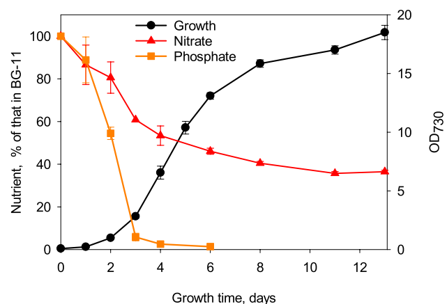
Fig. 1 Growth and uptake of nitrate and phosphate from BG-11 growth medium. The growth of Synechocystis culture was monitored once a day by measuring \text{OD}_{730} , and the amounts of remaining nitrate and phosphate in BG-11 growth medium were also measured daily. The nitrate concentration of BG-11 is 17.6 mM and phosphate concentration is 0.175 mM. The pH of the BG-11 growth medium was buffered by adding 20 mM HEPES–NaOH, pH 7.5, and the control strain cells were grown under constant illumination, PPFD 40 \mu\text{mol m}^{-2} \text{s}^{-1} , at 32^\circ\text{C} . The growth chamber air was enriched with 3% \text{CO}_2 . Three independent biological replicates were measured, and the error bars denote SE
