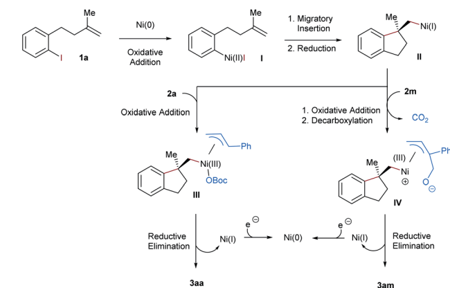
Scheme 4 Proposed mechanism.
