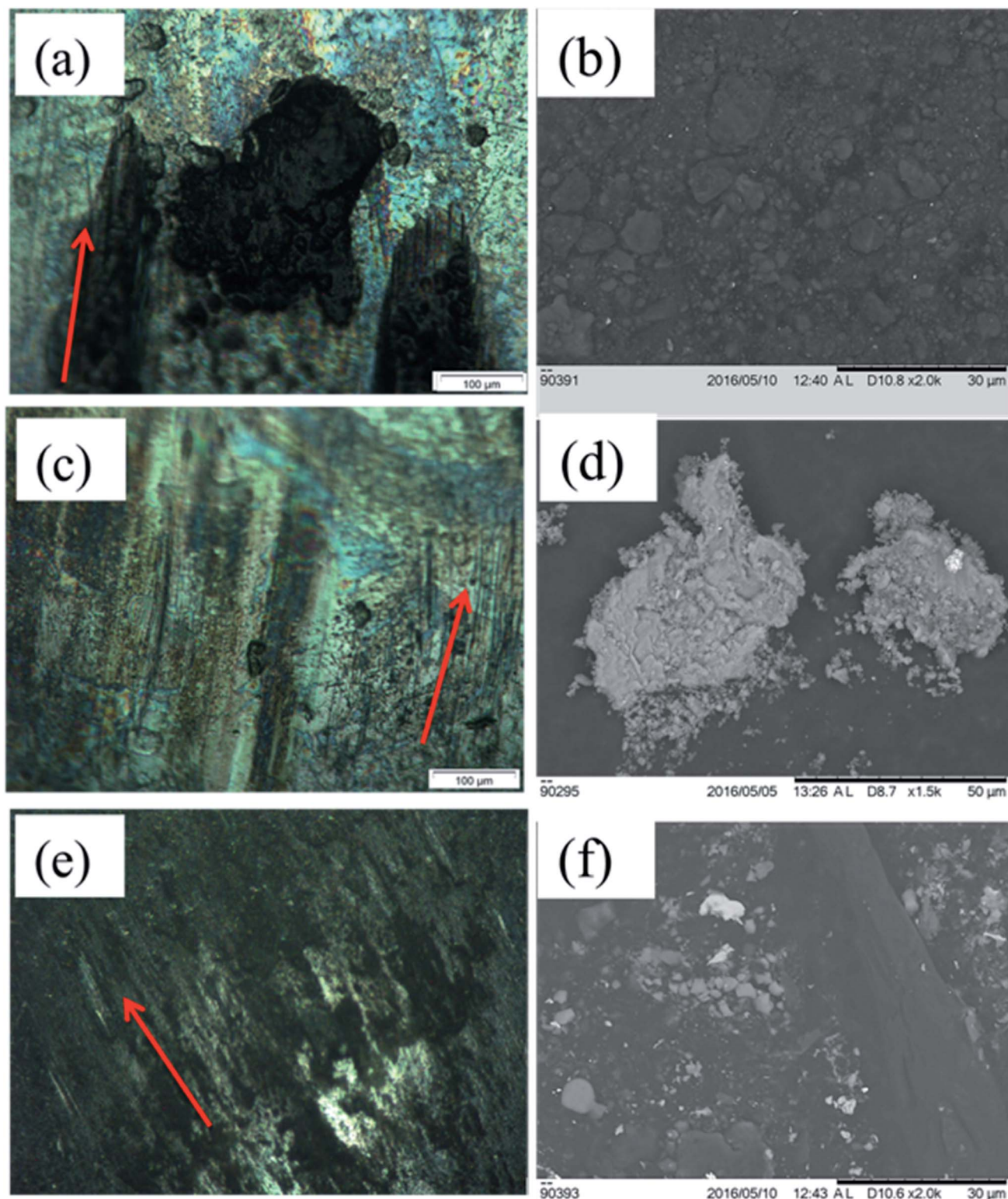
Fig. 9 Optical micrographic images of counter-body worn tracks and SEM images of worn debris for (a), (b) 5 wt% graphite (c), (d) 10 wt% graphite, (e), (f) 15 wt% graphite respectively.
