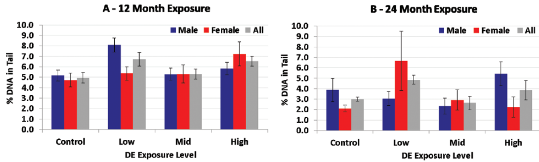
Figure 3. %DNA tail data from modified comet assay in rat lung tissue. (A) For 12-month exposure group. (B) For 24-month-exposure group. Data shown are the mean %DNA ± SEM; P > .05 , number of animals, data normalization, and DE exposure levels are as described in Figure 1. DE indicates diesel exhaust.
