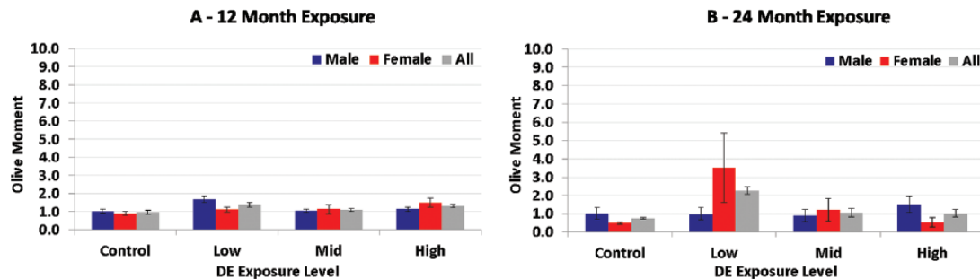
Figure 4. Olive moment data from modified comet assay in rat lung tissue. (A) For 12-month exposure group. (B) For 24-month exposure group. Data shown are the mean olive moment ± SEM; P > .05 , number of animals, data normalization and DE exposure levels are as described in Figure 1. DE indicates diesel exhaust.
