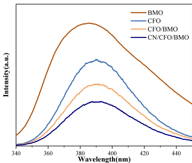
Fig. 7 The PL spectra of \text{CoFe}_2\text{O}_4 , \text{Bi}_2\text{MoO}_6 , and the \text{CoFe}_2\text{O}_4/\text{Bi}_2\text{MoO}_6 , g\text{-C}_3\text{N}_4/\text{CoFe}_2\text{O}_4/\text{Bi}_2\text{MoO}_6 composites.
