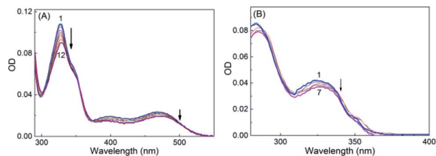
Fig. 1 (A) Absorption spectra of sanguinarine at different concentrations of SBE 7 \beta CD at pH 6.5. [SBE 7 \beta CD]/ \mu\text{M} : (1) 0.0, (2) 1.8, (3) 3.6, (4) 9.7, (5) 24.1, (6) 43.0, (7) 65.3, (8) 94.0, (9) 149.0, (10) 208.6, (11) 275.0 and (12) 360.0. (B) Absorption spectra of sanguinarine at different concentrations of SBE 7 \beta CD at pH 10. [SBE 7 \beta CD]/ \mu\text{M} : (1) 0, (2) 24, (3) 50, (4) 99, (5) 196, (6) 990 and (7) 1234.
