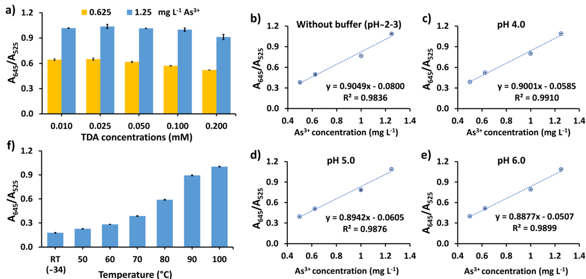
Fig. 4 (a) Effect of TDA concentration on the detection of \text{As}^{3+} at 0.625 and 1.25 \text{mg L}^{-1} , (b–e) effect of pH (3.0 to 6.0) of 5 mM Britton–Robinson buffer on the sensitivity of the linear plot between the A_{645}/A_{525} ratio and \text{As}^{3+} ranging from 0.5 to 1.25 \text{mg L}^{-1} , and (f) the effect of reaction temperature on the detection of \text{As}^{3+} at 1.0 \text{mg L}^{-1} .
