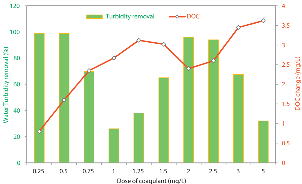
Fig. 3. Effects of the coagulant dose on water turbidity removal and DOC change in treated water.
