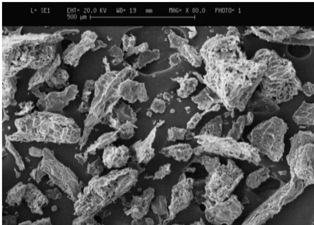
Fig. 1. The SEM image of sludge after water turbidity removal by the coagulant extracted from Plantago ovata seeds.
