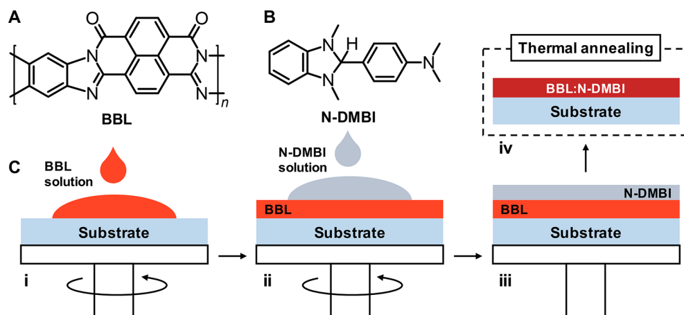
Figure 1. Chemical structures of (a) BBL and (b) N-DMBI. (c) Schematic illustration of the sequential doping process: (i) spin-coating of BBL; (ii) spin-coating of N-DMBI; (iii) resulting bilayer; and (iv) thermal annealing at different temperatures.
