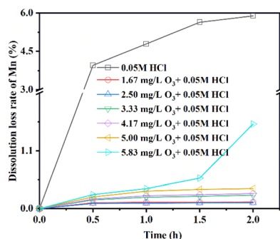
Fig. 6 The MDL of LMO under 0.05 \text{ mol L}^{-1} \text{ HCl} + R \text{ mg L}^{-1} \text{ O}_3 ( R = 0, 1.67, 2.50, 3.33, 4.17, 5.00, \text{ and } 5.83 ).
