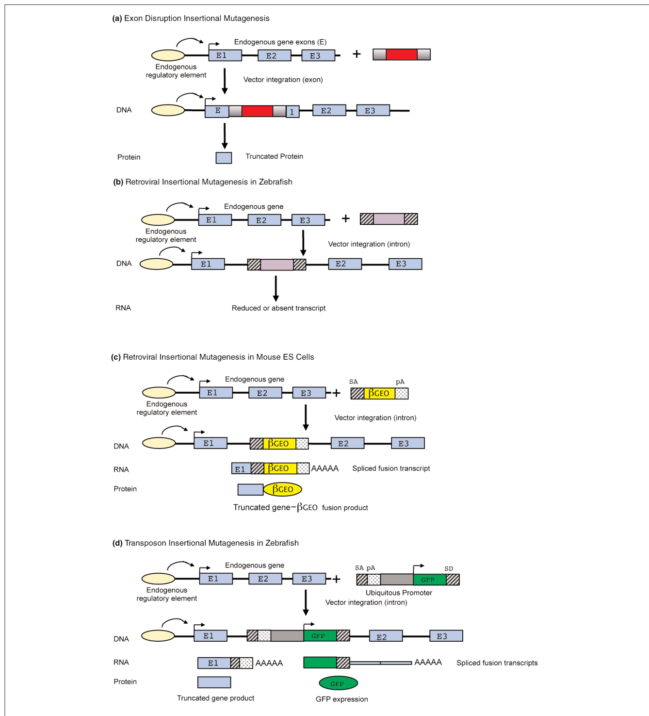
Figure 1 Insertional mutagenesis strategies used in vertebrates. In each case, a schematized endogenous locus is represented by exons (E) and an endogenous regulatory element. A nonintegrated vector is also shown above, with integrated vector below. Transcriptional start sites are shown as an arrow above each diagram. (a) Integration of DNA into a coding exon can mutate the locus, resulting in a truncated gene product. (b) Retroviral insertional mutagenesis alters the tagged locus using multiple methods, including the loss of the encoding transcript. (c) 5' gene trapping in mouse embryonic stem cells. Shown is one approach whereby the resulting fusion transcript encodes a truncated gene product fused to the selectable marker protein. (d) Insertional mutagenesis in zebrafish using transposons. Based on 3' exon or poly(A) trapping methods, this approach uses two components: a transcriptional termination cassette to truncate the integrated locus and a separate 3' exon trap gene finding cassette. See text for details. pA, polyadenylation signal; SA, splice acceptor; SD, splice donor.
