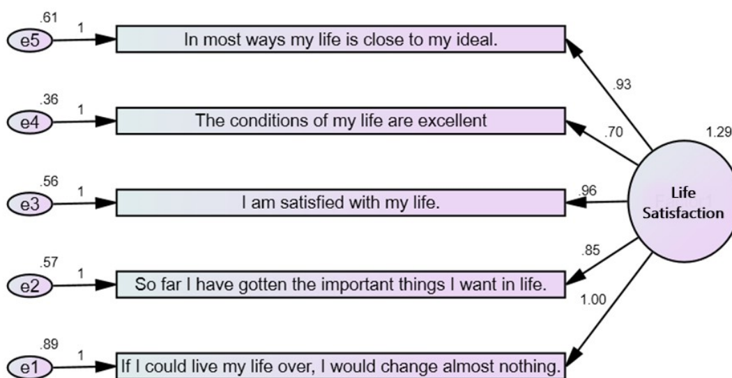
Fig 1. Single-factor Model of SWLS
