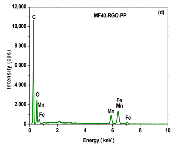
Figure 6. (a) FE-SEM image of cross-sections of MF20-RGO-PP, (b) EDX spectrum of MF20-RGO-PP, (c) FE-SEM image of cross-sections of MF40-RGO-PP and (d) EDX spectrum of MF40-RGO-PP.
