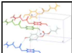
Fig. 2. A part of the crystal structure of the title compound, including hydrogen bonds depicted with blue dashed lines, and C—H... \pi contacts from the asymmetric unit, represented as red dashed lines. Colour code for symmetry-related molecules: blue -x, -1/2+y, -z ; green -x, 1/2+y, -z ; red 1-x, 1/2+y, -z ; gold x, 1+y, z .
