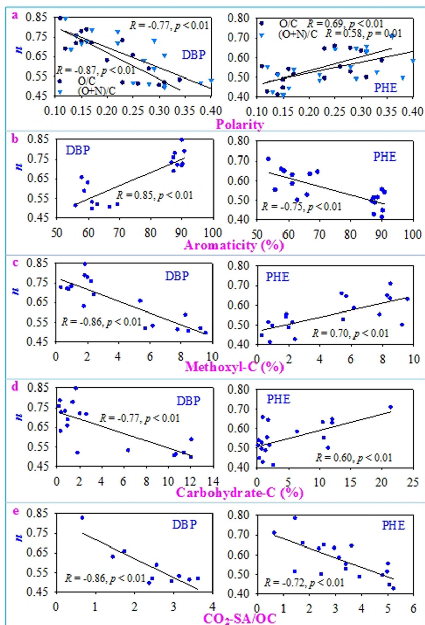
Figure 6 | Correlations between the Freundlich nonlinearity coefficients ( n ) of DBP and PHE sorption isotherms of DBP and PHE by the biochars and the polarity ( (N + O)/C and O/C ) (a), and contents of the aromaticity (b), methoxyl-C (c), and carbohydrate-C (d) obtained by ^{13}C -NMR, and organic carbon (OC)-normalized surface area as determined by CO_2 adsorption ( CO_2 -SA/OC) (e) of the biochars.
