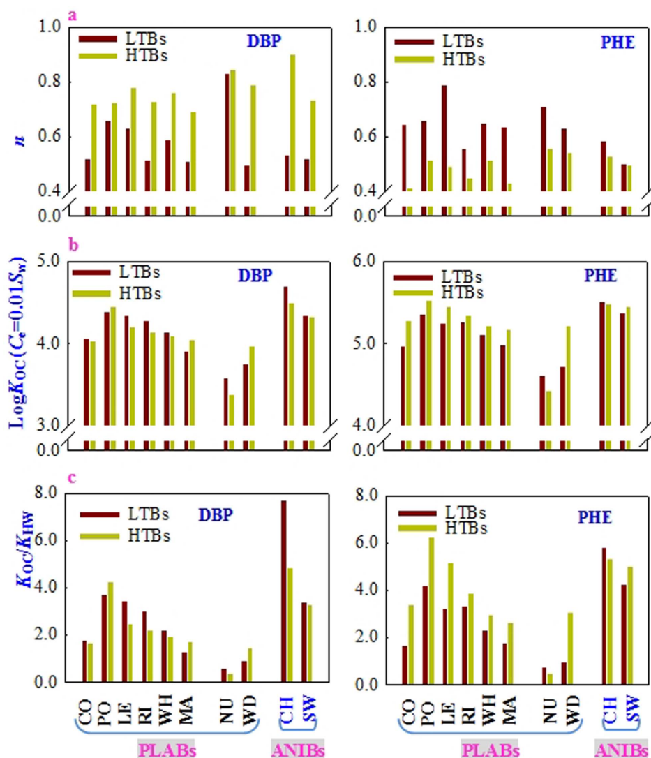
Figure 3 | Comparison of Freundlich nonlinearity coefficients ( n ) of DBP and PHE sorption isotherms (a), sorption capacity as indicated by the organic carbon (OC)-normalized distribution coefficient ( \log K_{OC} , mL g -1 ) (b), and the K_{HW} -normalized K_{OC} values ( K_{HW} , hexadecane-water partition coefficient) of DBP and PHE between the LTBs and HTBs (c). CO, PO, LE, RI, WH, MA, NU, WD, CH and SW refer to the biochars produced from cotton straw, potato straw, leaf, rice straw, wheat straw, maize straw, nut, wood dust and manures of chicken and swine, respectively. LTB and HTB represent the biochars obtained under pyrolysis or heat treatment temperature (HTT) at 300 and 450°C, respectively.
