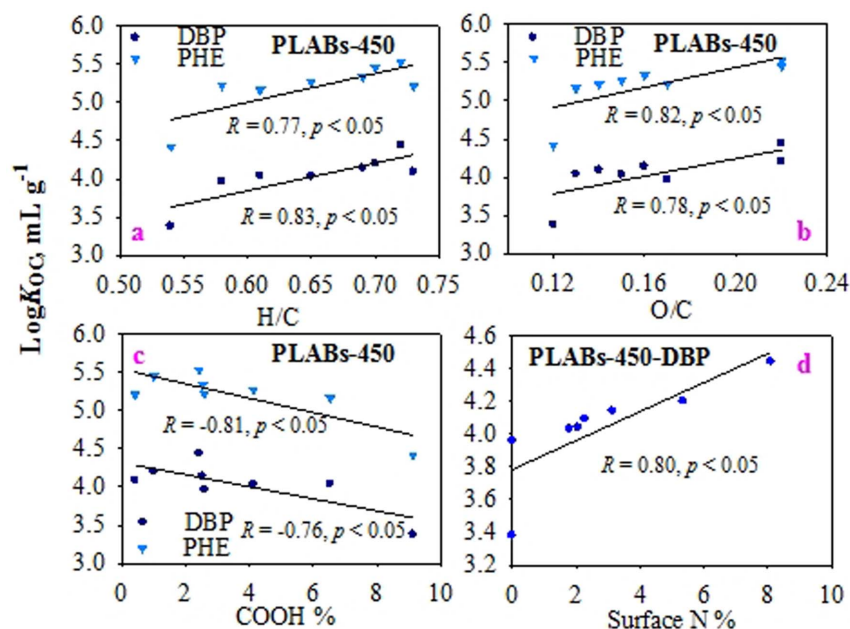
Figure 5 | Correlations between organic carbon (OC)-normalized sorption distribution coefficient ( \log K_{OC} , C_e = 0.01S_w (the solubility of DBP or PHE in water at 20 °C)) of DBP and PHE by plant-derived biochars at 450 °C (PLABs-450) and the atomic ratios of H/C (a) and O/C (b), the percentages of COOH (c) determined by XPS results, and surface content of N (d).
