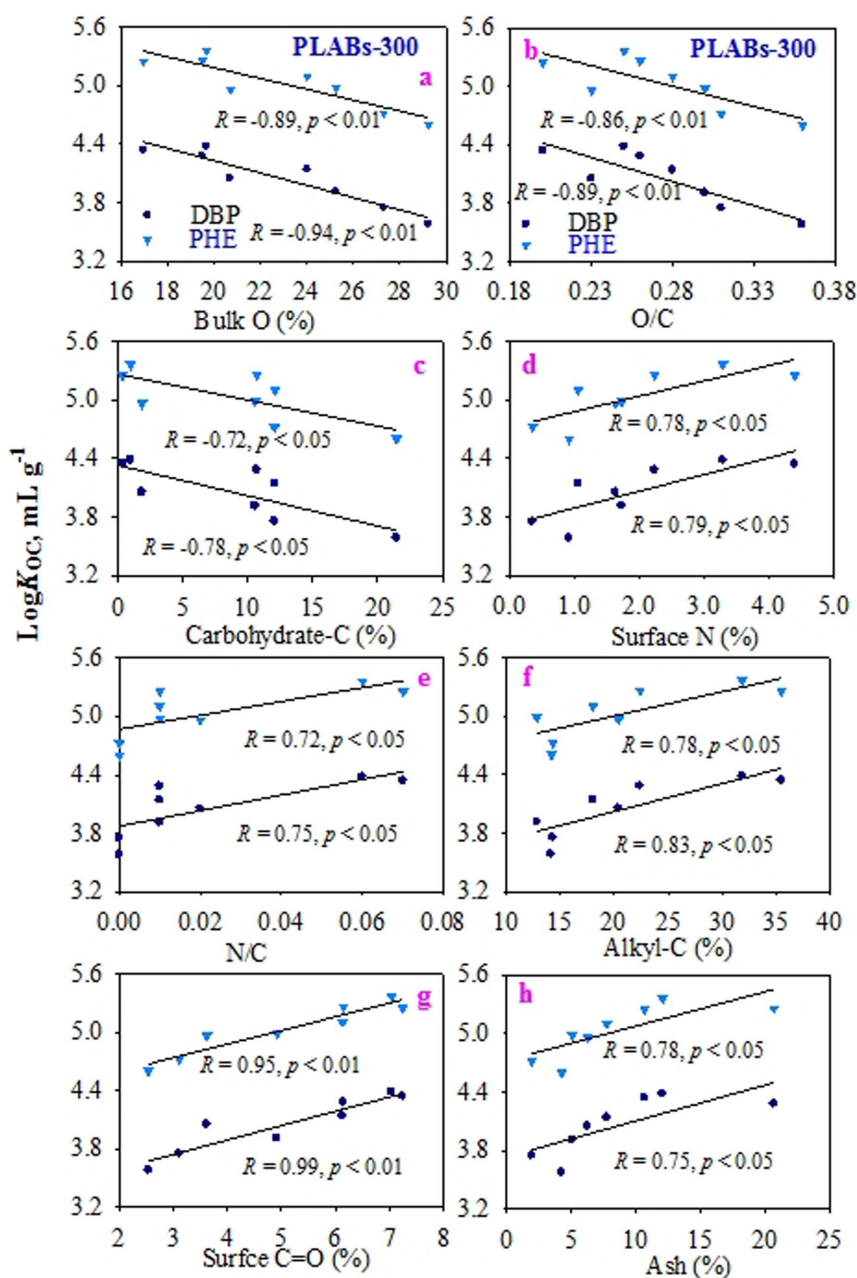
Figure 4 | Correlations between the organic carbon (OC)-normalized sorption distribution coefficient ( \log K_{OC} , C_e = 0.01S_w (the solubility of DBP or PHE in water at 20 °C)) of DBP and PHE by the plant-derived biochars at 300 °C (PLABs-300) and the content of bulk O (a) and bulk atomic ratio of O/C (b) as determined by the elemental analysis, carbohydrate-C (c) according to the ^{13}\text{C} -NMR results, the content of surface N (d) as indicated by XPS results, the bulk atomic ratio of N/C (e), the content of alkyl-C (f), the content of surface polar group of C=O (g), and the ash content (h) of PLABs-300.
