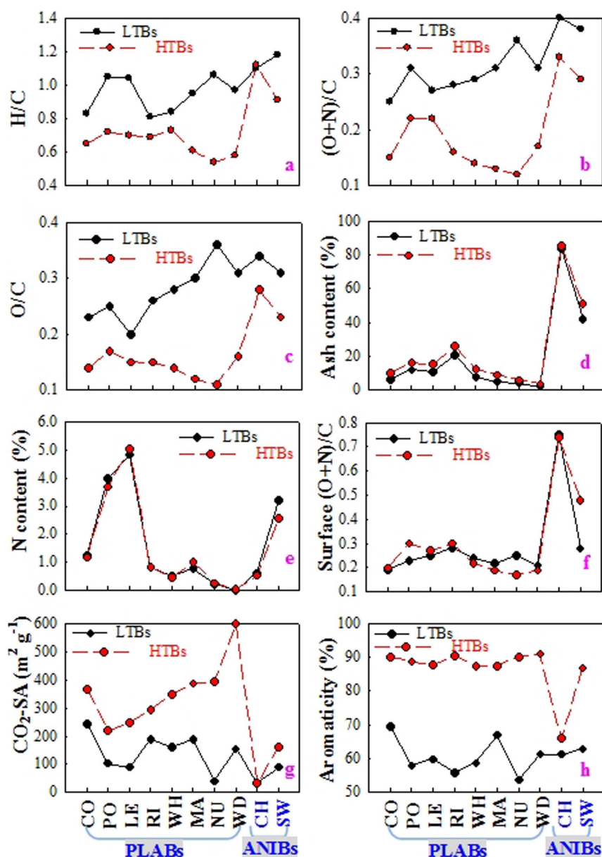
Figure 1 | Comparison of H/C atomic ratio (a), bulk polarity ((O + N)/C) (b), O/C atomic ratio (c), ash content (d), N content (e), surface polarity ((O + N)/C) (f), surface area determined by CO 2 adsorption (CO 2 -SA) (g), and aromaticity (h) between the low-temperature biochars (LTBs) and high-temperature biochars (HTBs). CO, PO, LE, RI, WH, MA, NU, WD, CH and SW refer to the biochars produced from cotton straw, potato straw, leaf, rice straw, wheat straw, maize straw, nut, wood dust and manures of chicken and swine, respectively. Plant-residues and animal-waste derived biochars were named by PLABs and ANIBs, respectively. LTB and HTB represent the biochars obtained under pyrolysis or heat treatment temperature (HTT) at 300°C and 450°C, respectively.
