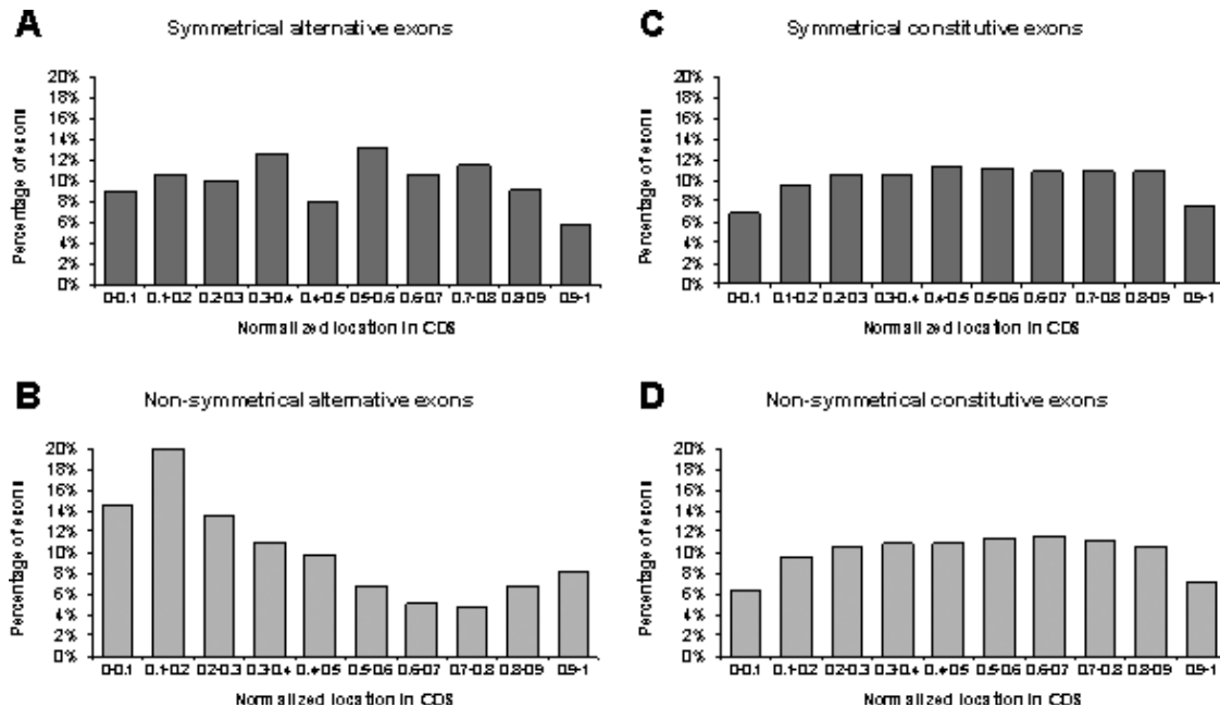
Figure 4. Percentage of symmetrical and non-symmetrical exons along the CDS. (A–D) Percentage of exons in different locations along the CDS, in increments of 0.1 (exon locations in CDS are normalized between 0 and 1, see Supplementary Data). A and B show the distribution of alternative exons, C and D show that of constitutive exons.
