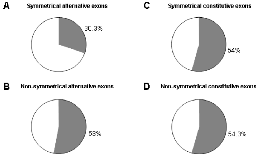
Figure 2. Percentage of exons that overlap with protein domain coding sequence. Gray and white indicate the fraction of exons that encodes protein domain fragments or full domains and those that do not encode for any fragment of a protein domain, respectively. (A) and (B) are for alternatively spliced exons, (C) and (D) are for constitutively spliced ones.
