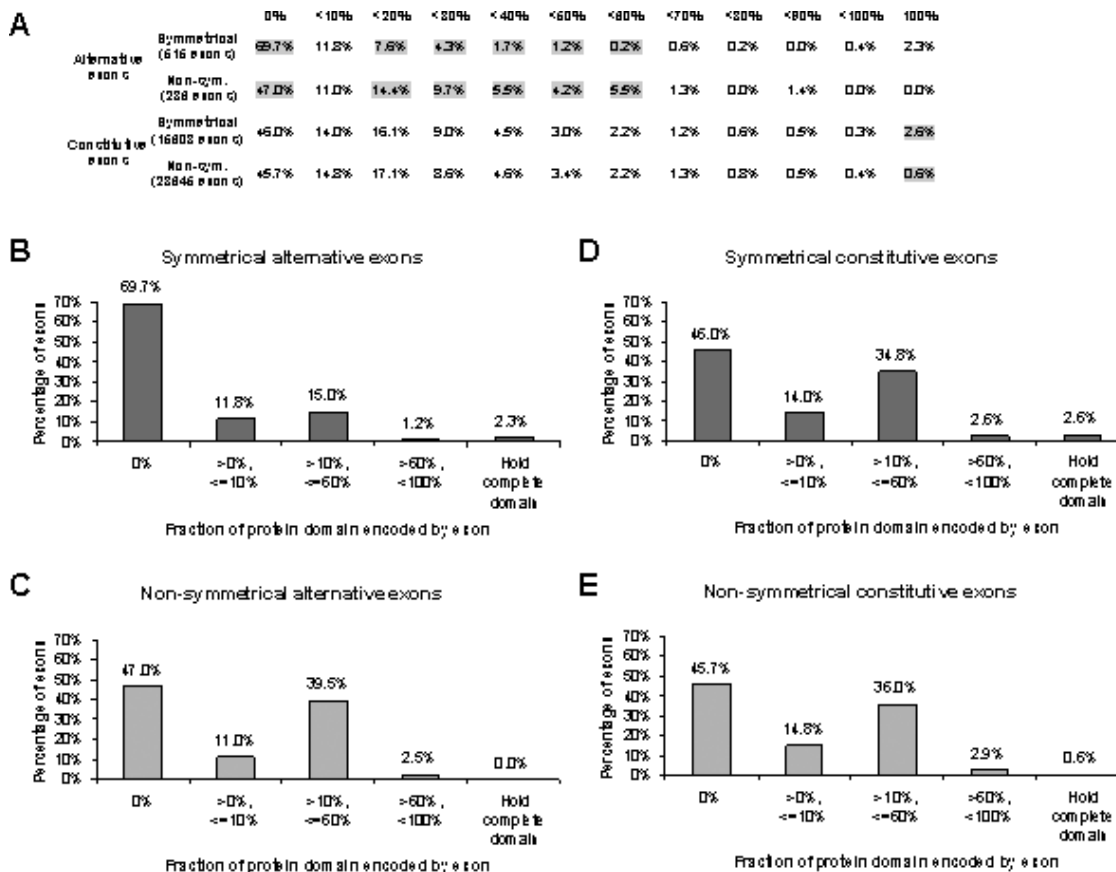
Figure 3. Percentage of symmetrical and non-symmetrical exons that encode different fractions of protein domains. (A) The percentage of symmetrical and non-symmetrical alternative and constitutive exons that encode for different fragments of protein domains, starting with exons not encoding any domain fragment (0%), then encoding different sizes of fragments (in increments of 10%) up to encoding complete domains (the bar marked 100%). Statistically significant differences between symmetrical and non-symmetrical alternative exons and between symmetrical and non-symmetrical constitutive exons are highlighted in gray. (B–E) A histogram representation of the results shown in (A), indicating the percentage of exons that do not encode protein domains (0%), encodes more than 0% and up to 10% of protein domains ( >0\% , \leq 10\% ), encodes medium-sized fragments ( >10\% , \leq 60\% ), encodes fragments that consist of >60\% and <100\% of protein domains or holds complete domains. B and C show the distribution of alternative exons, D and E show that of constitutive exons.
