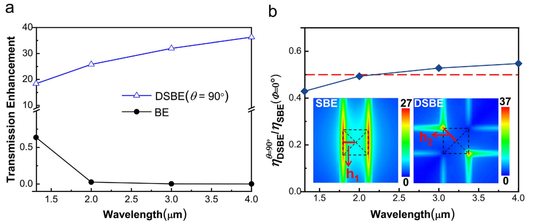
Figure 5. Comparison of transmission enhancement between DSBE antennas and BE/SBE antennas. (a) Transmission enhancement of DSBE ( \theta = 90^\circ ) and BE antennas at \lambda = 1.31, 2.0, 3.0, and 4.0 \mu\text{m} , and the corresponding film thicknesses h = 0.38, 0.64, 1.07, and 1.48 \mu\text{m} , respectively. (b) The ratio of \eta_{\text{DSBE}}^{\theta=90^\circ} / \eta_{\text{SBE}} (\Phi = 0^\circ) from 1.31 to 4 \mu\text{m} . The red dashed line corresponds to the value of 0.5 . The inserts are the normalized and time-averaged |E| intensity distributions of SBE and DSBE antennas on the z = 0 plane at \lambda = 1.31 \mu\text{m} with \Phi = -\theta/2 .
