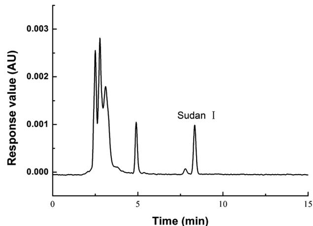
Fig. 6 HPLC-UV chromatogram of a typical soybean oil sample. Detected wavelength is 478 nm.
