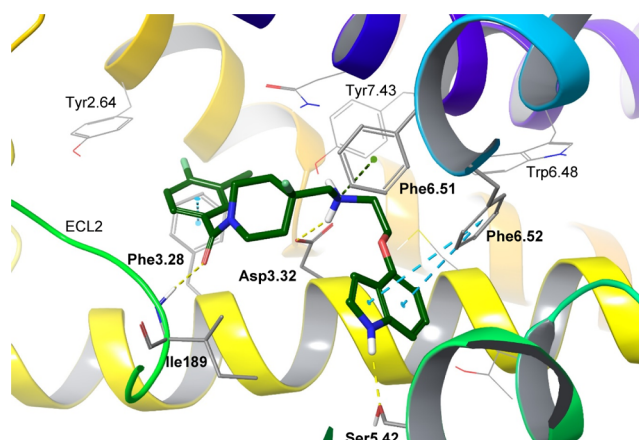
Figure 4. Predicted binding mode of compound 56 (with HBD in meta position) in the site of the serotonin 5-HT 1A receptor. Amino acid residues engaged in ligand binding (within 4 Å from the ligand atoms) are displayed as sticks, whereas crucial residues, for example, forming H-bonds (dotted yellow lines), \pi - \pi /CH- \pi stacking (dotted cyan lines), and cation- \pi interactions (dotted green line) are represented as thick sticks. ECL2 residues were hidden for clarity; ECL—extracellular loop. The homology model of the 5-HT 1A receptor is based on the crystal structure of the 5-HT 1B receptor (PDB ID: 4IAR).
