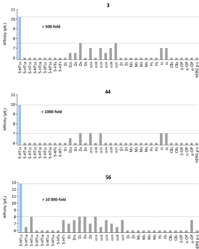
Chart 1. Graphical Visualization of Selectivity Profiles of Compounds 3, 44, and 56 a
