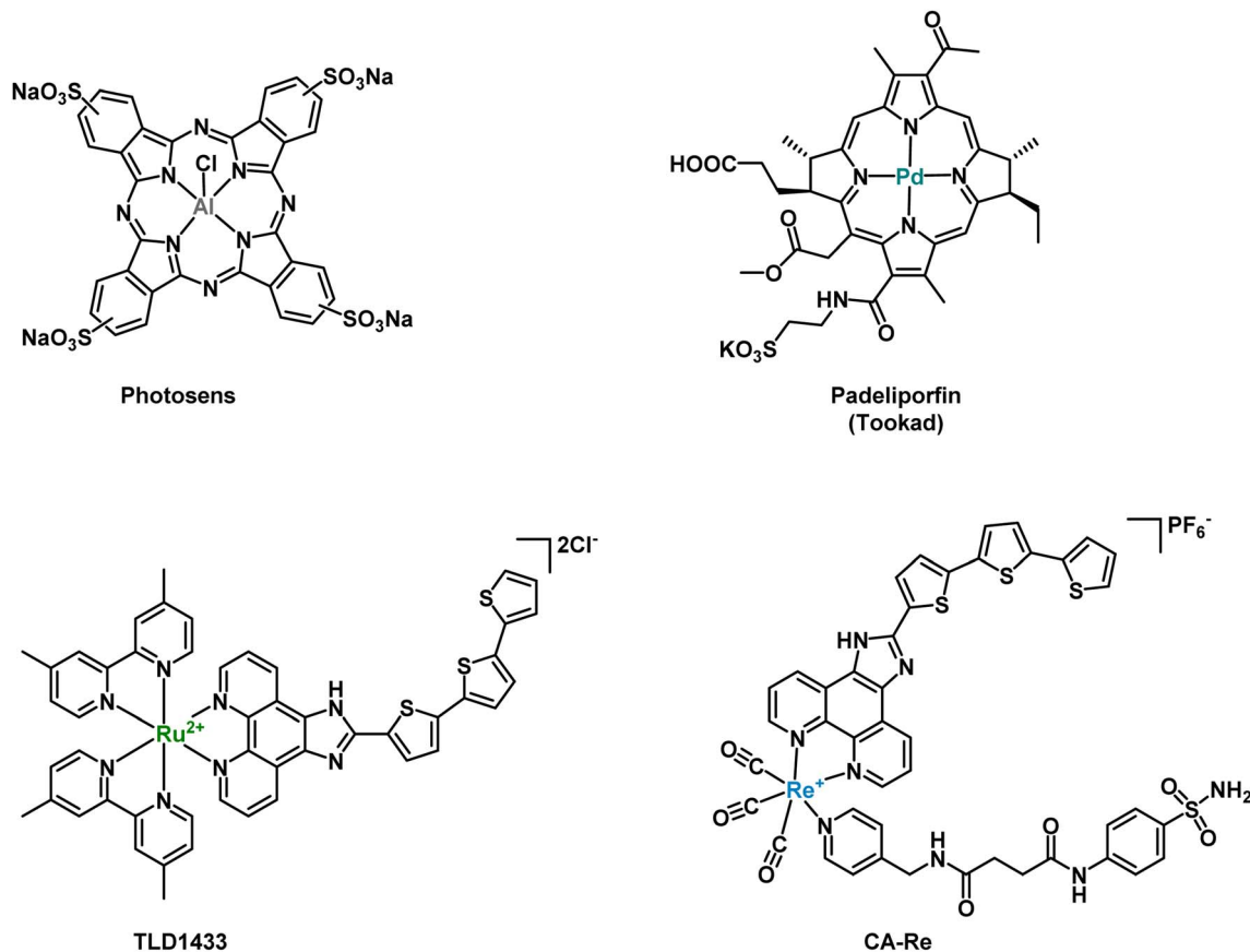
Fig. 1 Metal-based PDT PS, which have been approved or are currently in clinical trials, and rhenium-CA inhibitor based PDT PS developed by Mao et al. 48
