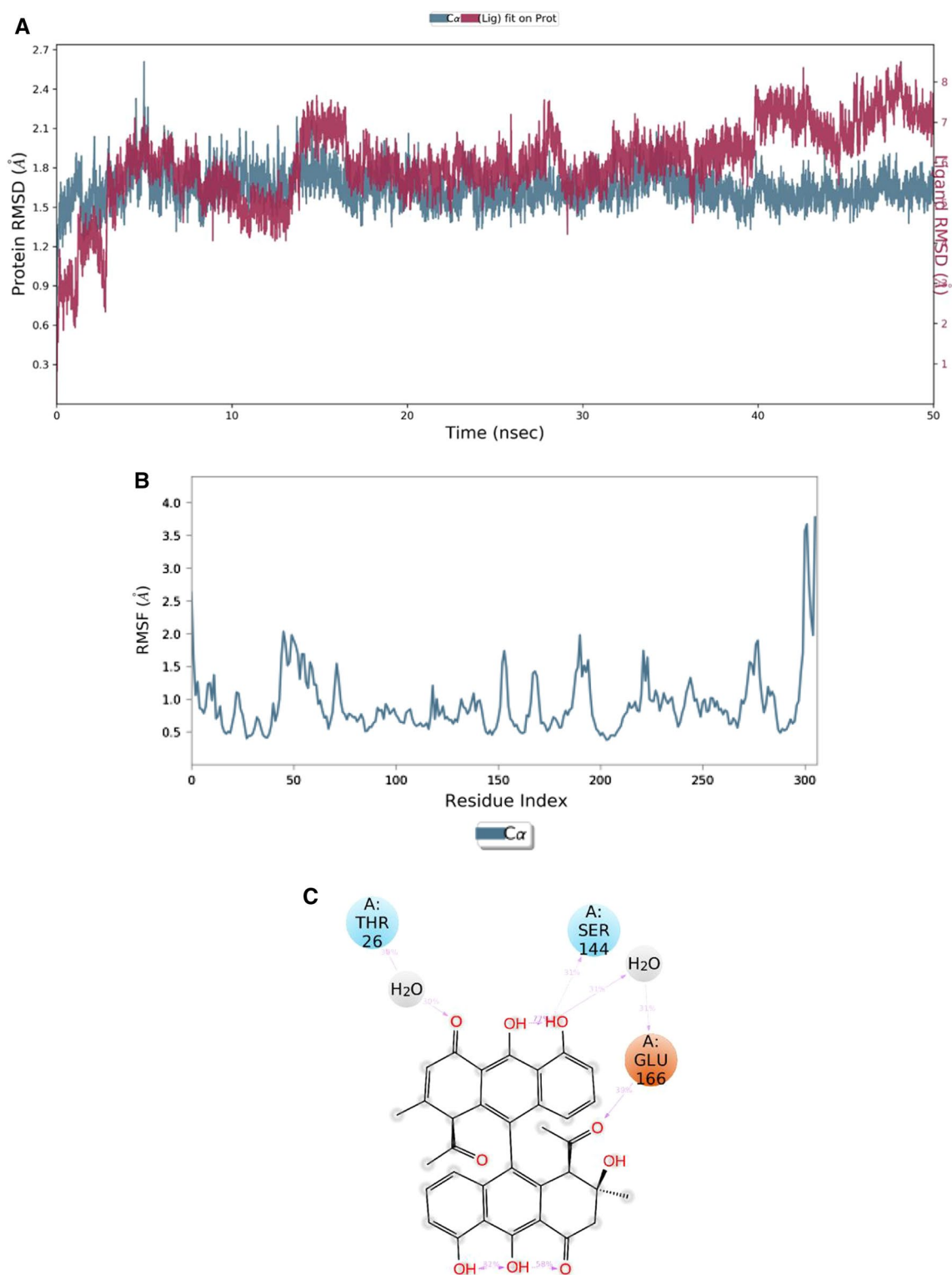
Fig. 3 A Root mean square deviation, B root mean square fluctuation of SARS-CoV-2 M^{pro} C \alpha and inhibitor setomimycin during 50 ns of MD simulation. C SARS-CoV-2 M^{pro} -setomimycin 2D interaction diagram. The interactions persisting more than 30% of total simulation time were shown. The pink arrow indicates hydrogen bonding
