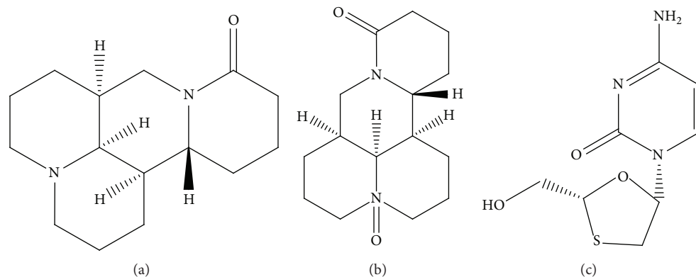
FIGURE 1: The chemical structures of matrine (a), oxymatrine (b), and lamivudine (c).
