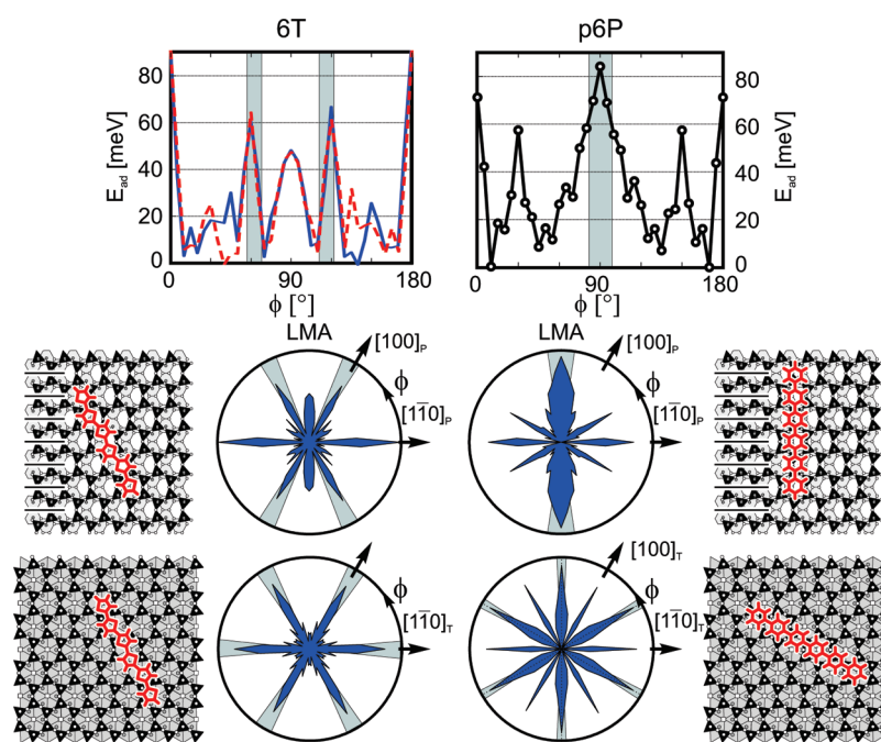
Figure 5. Adsorption energy of 6T (left) and p6P (right) on pyrophyllite as a function of angle \phi . The zero on the energy scale is set to the energy of the least favorable angle. For 6T, two curves are shown, one corresponding to left-handed and the other to right-handed molecules. Middle: Polar diagrams of the adsorption energy of 6T (second from left) and p6P (second from right) on pyrophyllite. As described in the text, for 6T the two curves are merged into one. The left-most and right-most plots depict the experimentally confirmed adsorption geometries. Bottom: Polar diagrams of the adsorption energy of 6T (second from left) and p6P (second from right) on talc and the experimentally confirmed adsorption geometries. Gray areas in the polar plot indicate molecular orientations which have been experimentally observed.
