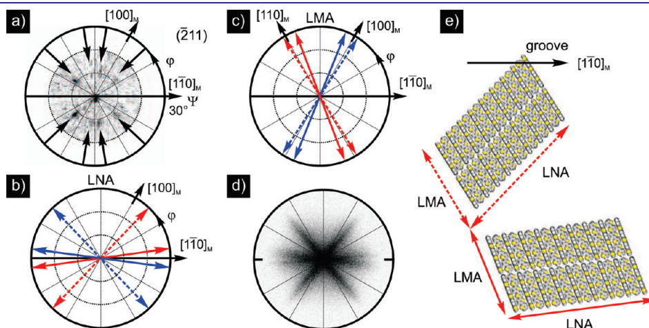
Figure 3. (a) XRD pole figure measurement of 6T nanofibers grown on muscovite mica. Arrows indicate the determined position of (\bar{2}11) reflexes. (b) Azimuthal alignment of the long needle axes (LNAs) deduced by XRD. (c) Angular alignment of the long molecular axes (LMAs). LMAs can be grouped into two pairs (red and blue) which are aligned quasi-parallel to each other. (d) FFT pattern calculated from an optical microscope image providing a perfect match with LNAs deduced by XRD. (e) Real space model of two 6T crystallites as deduced by XRD. Two LNAs originating from one molecular orientation (red arrows) are shown (6T crystallites mirrored due to substrate surface symmetry are not indicated).
