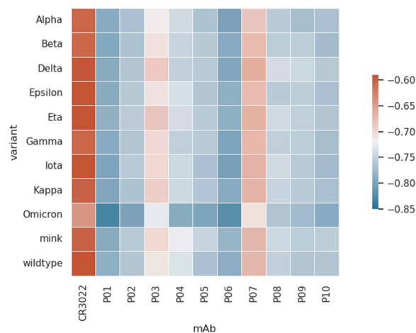
Fig. 6. Heatmap with the minima free energy of interactions values ( \beta w_{min} in KBT units) for the SARS-CoV-2 RBD-mAbs complexation at pH 7 and 150 mM of NaCl by the CpH MC simulations (FORTE) for the RBD of the main critical variants and different Rosetta-designer binder candidates (P01 to P10). The reference is the native fragment of CR3022. All values of. The maximum estimate error is 0.01. See the text for a description of mutations considered in each case.
