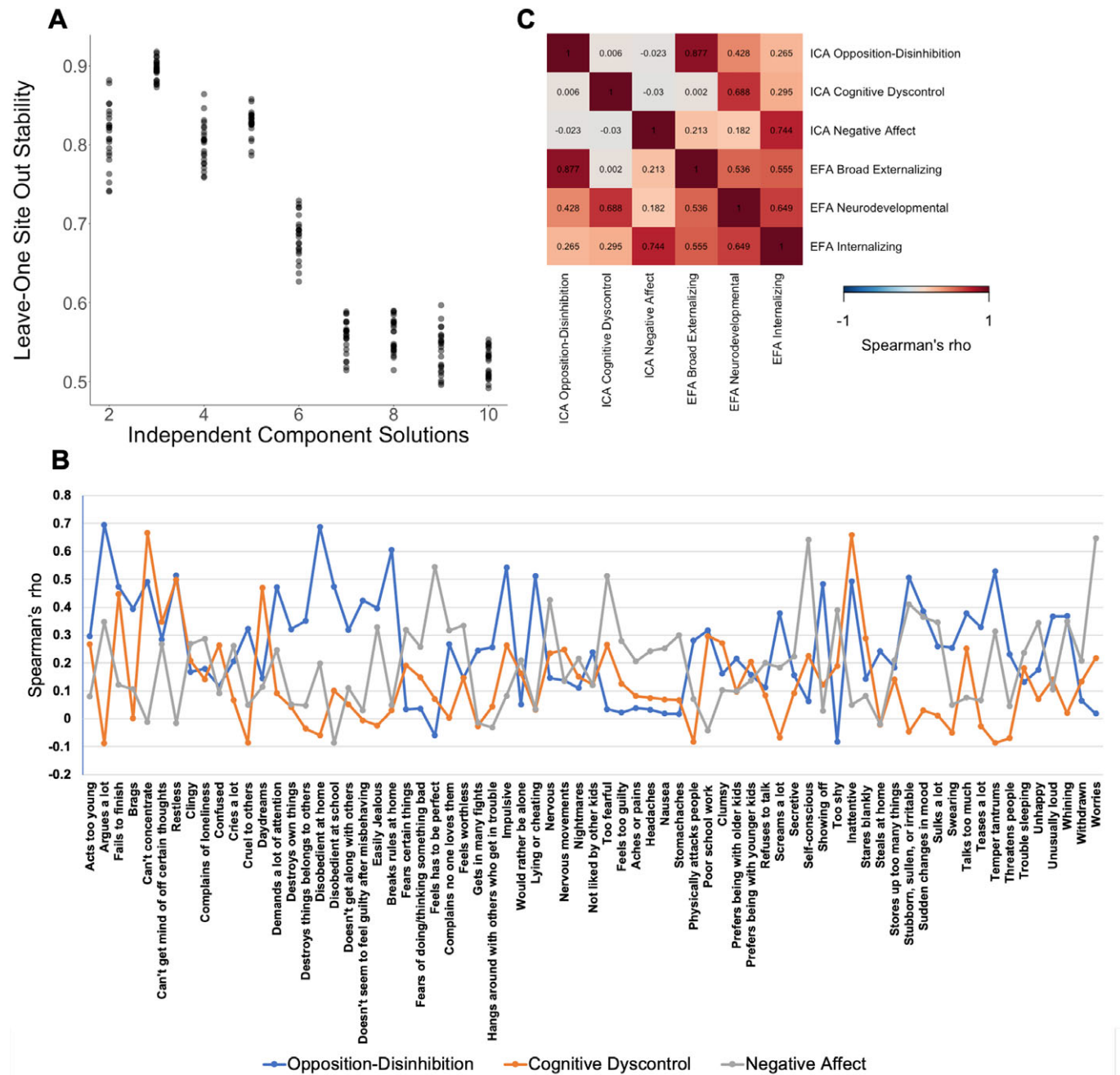
Figure 1. Data-driven structure of psychopathology in the ABCD dataset captured independent component analysis (ICA). A. Leave-one site stability for ICA solutions from 2-10 components; B. Item loadings on each independent component for the three-IC solution; C. Correlation between the three-IC solution and corresponding EFA-derived factors.
