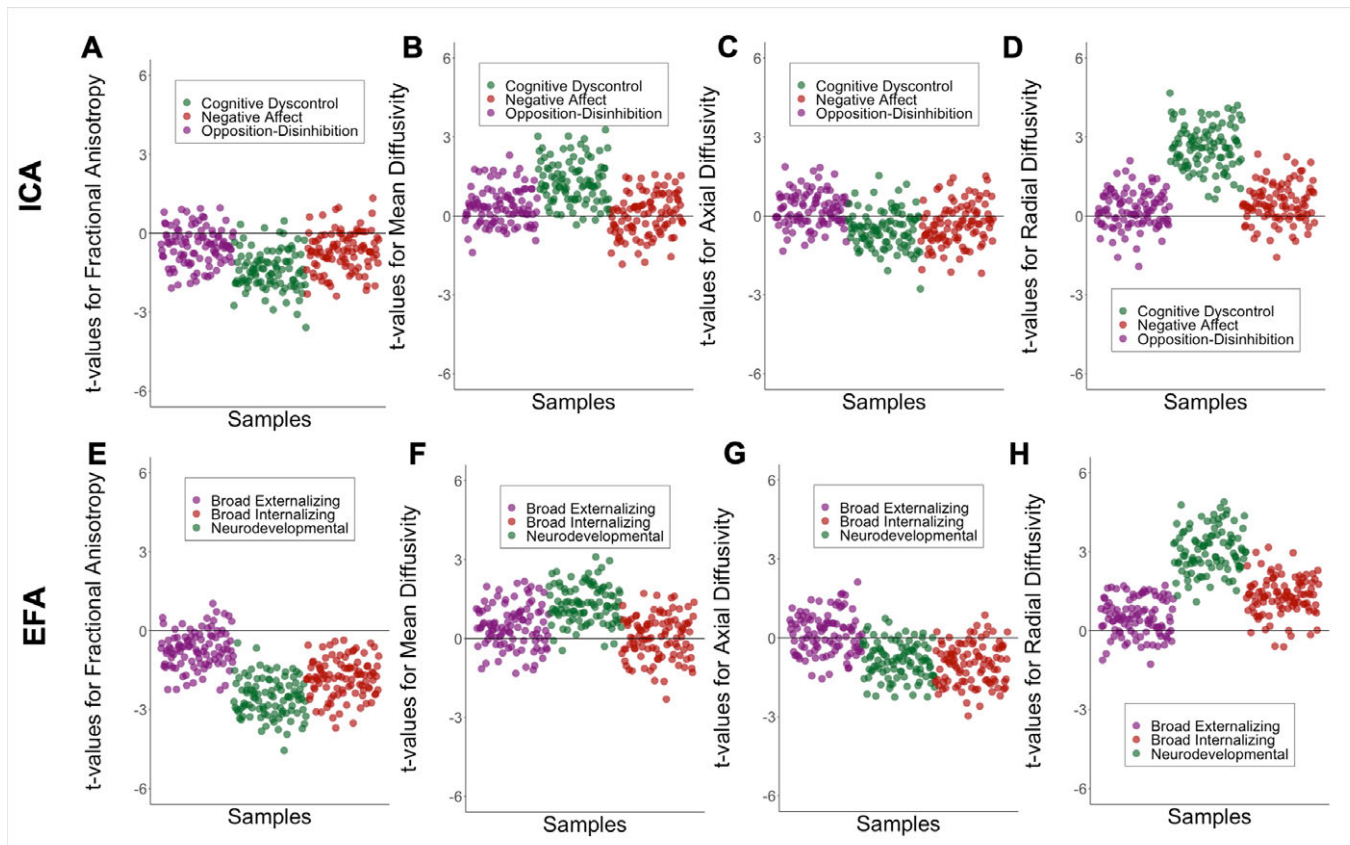
Figure 4. Association between global measures of white matter integrity and the most stable ICA solution, and three corresponding EFA factors using kernel regularized least squares (KRLS). Values represent t-value for the association between the measures of white matter integrity and psychopathology dimensions in 100 randomly resampled dataset of 50% original sample size; All analyses were adjusted for sex, age, and race, handedness, scanner, weight, height, pubertal stage, and head motion; A,B,C,D. Association between measures of white matter integrity and ICA-derived opposition-disinhibition, cognitive dyscontrol, and negative affect dimensions. E, F, G, H. Association between measures of white matter integrity and EFA-derived broad externalizing, neurodevelopmental, and broad internalizing factors.
