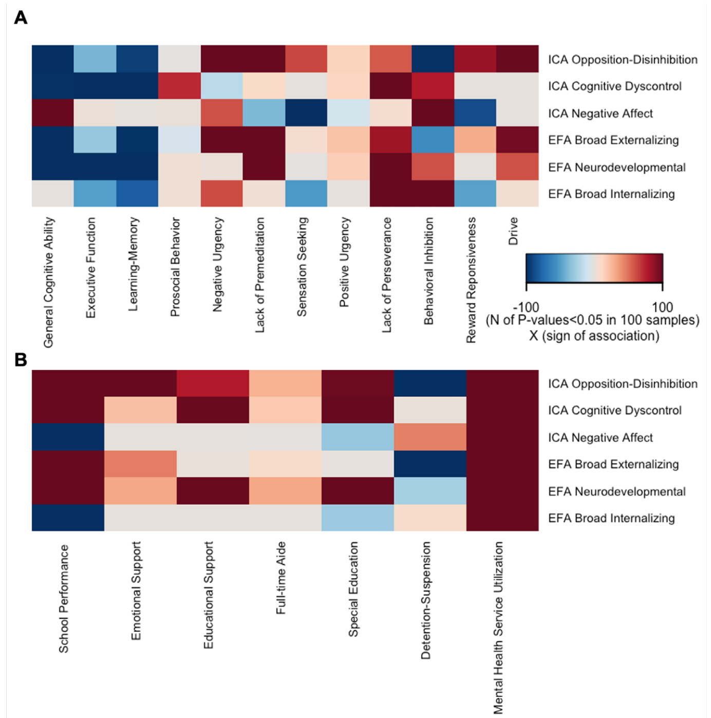
Figure 2. Validity of the Psychopathology Dimensions. Each cell represents number of FDR-corrected P-values < 0.05 in 100 reruns of the Kernel regularized least squares (KRLS) analysis on 50% randomly resampled data multiplied by the sign of the association. All analyses were adjusted for sex, race, age, and site; A. Association of psychopathology dimensions with cognitive and behavioral measures; for each psychopathology dimension, all measures are modeled together to characterize their independent contribution to psychopathology; B. Association of psychopathology dimensions with academic outcomes and service utilization; for each outcome, all three dimensions (ICA-derived or EFA-derived) are entered into the model together to quantify their independent contribution to the outcome.
