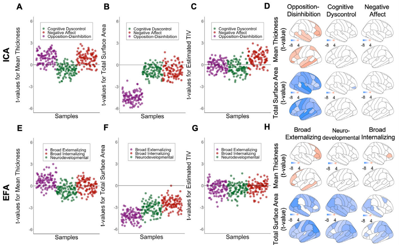
Figure 3. Association between global measures of brain morphometry and the most stable ICA solution, and corresponding EFA factors using kernel regularized least squares (KRLS); Values represent t-value for the association between morphometric brain measures and dimensions of psychopathology. For global measures, values represent t-values in 100 randomly resampled dataset of 50% original sample size. For regional measures values represent t-value from the model on the whole dataset; All analyses were adjusted for sex, age, and race, handedness, scanner, weight, height, pubertal stage; A, B, C Association between brain morphometric measures and ICA-derived opposition-disinhibition, cognitive dyscontrol, and negative affect dimensions. D, E, F. Association between brain morphometric measures and EFA-derived broad externalizing, neurodevelopmental, and broad internalizing factors.
