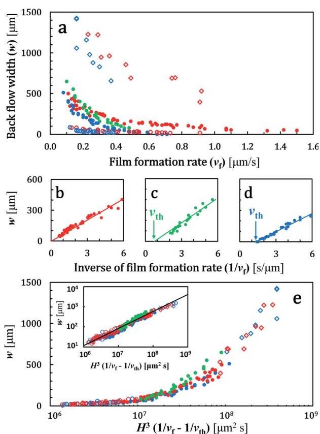
Fig. 3 (a) Width of the back-flow region ( w ) and film growth rate ( v_f ). Conditions ( d , \phi_w , H ) = (45 nm, 20 wt%, 100 \mu m) for red solid circles, (65 nm, 20 wt%, 100 \mu m) for green solid circles, (110 nm, 15 wt%, 100 \mu m) for blue solid circles, (45 nm, 20 wt%, 50 \mu m) for red open circles, (45 nm, 20 wt%, 200 \mu m) for red open squares, (110 nm, 15 wt%, 50 \mu m) for blue open circles, and (110 nm, 15 wt%, 200 \mu m) for blue open squares. Data of red, blue, and green solid circles in (a) are replotted by using v_f^{-1} in (b)–(d). The solid line in (b)–(d) show a linear fitting result for the data for v_f^{-1} < 6 [ s \mu m^{-1} ]. (e) All data in (a) were plotted by using H^3(1/v_f - 1/v_{th}) . The inset in (e) shows the same data in a log–log plot. The solid line in the inset shows a slope of 0.85. The same symbols as in (a) are used in (b)–(e).
