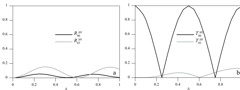
Figure 10. R_{00}^{SH} and R_{02}^{SH} (a) and T_{00}^{SH} and T_{02}^{SH} (b) as a function of \delta for r = 0.1 .
