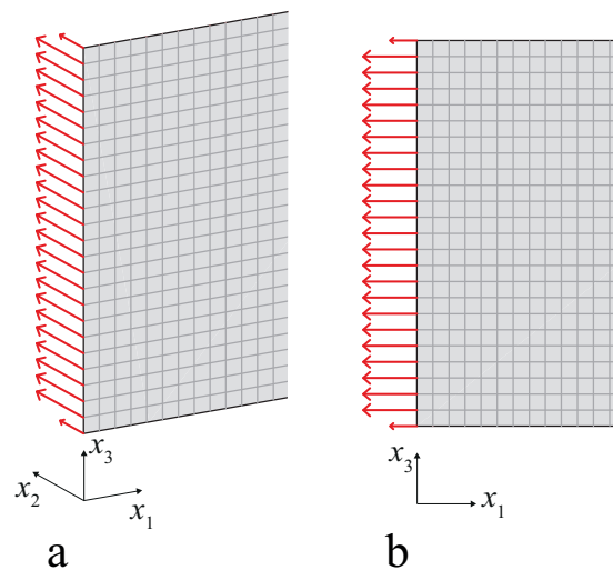
Figure 6. Spatial distribution of forces used to generate SH0 (a) and S0 (b) waves.
