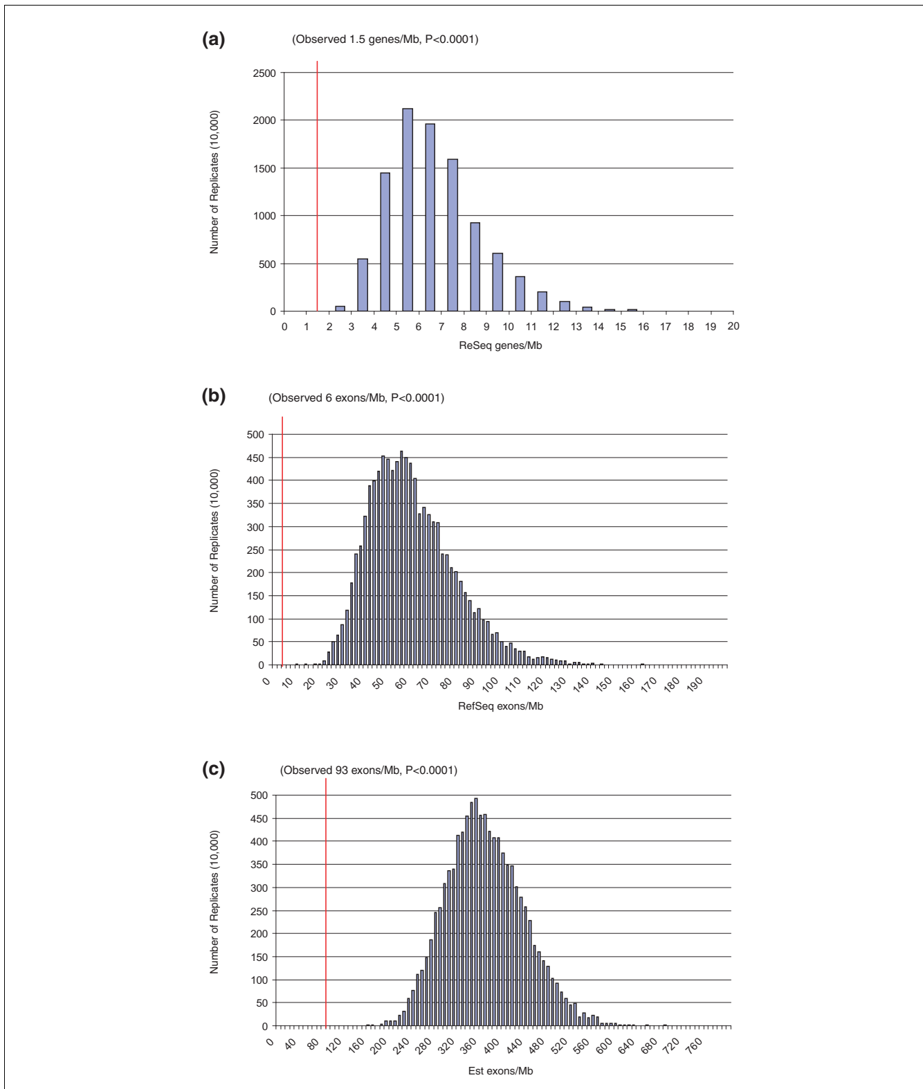
Figure 3 Gene density simulations. The observed density of (a) genes (Refseq), (b) Refseq exons and (c) expressed sequence tag (Est) exons within the corresponding region of the 14 ENCs were compared against a simulated set of 10,000 regions distributed randomly within the human genome (see Materials and methods). A significant depletion of exons and genes was observed.
