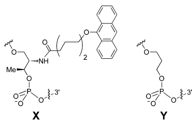
Figure 1. Structures of the nucleosidic groups X and Y when incorporated into DNA (phosphodiester groups toward 3' end).
