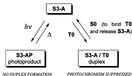
Scheme 2. Representation of Photocontrolled Binding of T0 and Binding-Controlled Photoreactivity within the S3-A \leftrightarrow S3-AP Photochromic System
