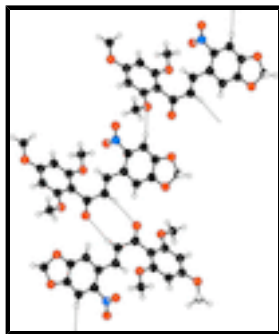
Fig. 2. A partial packing diagram. Hydrogen bonds are shown as dashed lines.
