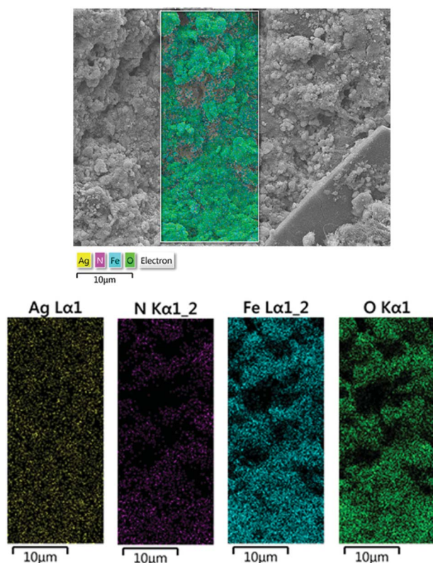
Fig. 6 Mapping analysis of the Fe 3 O 4 -MWCNTs@PEI-Ag composite.
